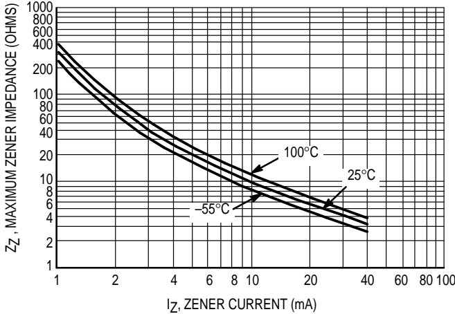
Figure 4. 1N821 Series
