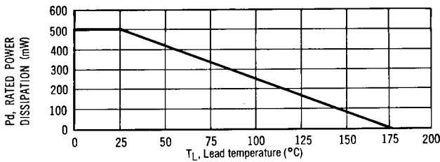
FIGURE 2 Power Derating Curve
