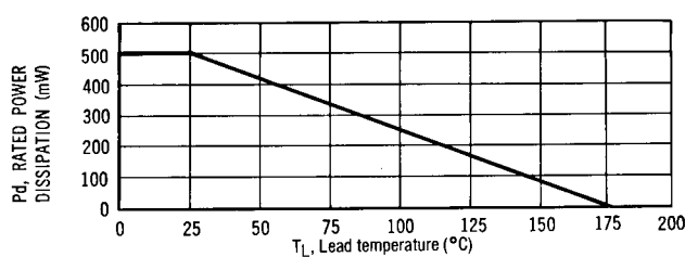
FIGURE 2 Power Derating Curve
