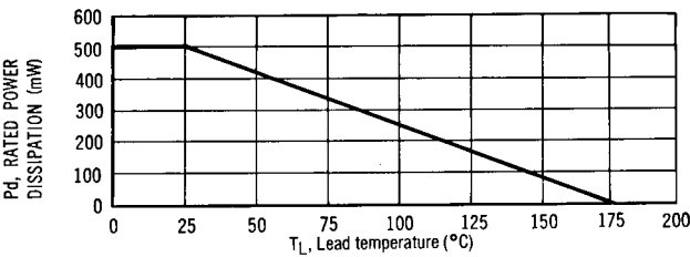
FIGURE 2 Power Derating Curve
