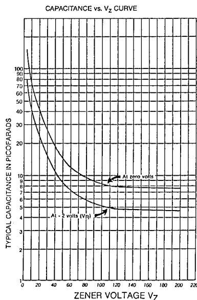
FIGURE 4 CAPACITANCE VS. ZENER VOLTAGE (TYPICAL)
