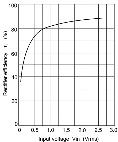
Fig.4 Rectifier efficiency Vs. Input voltage
