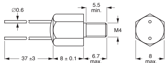
Component outline.
