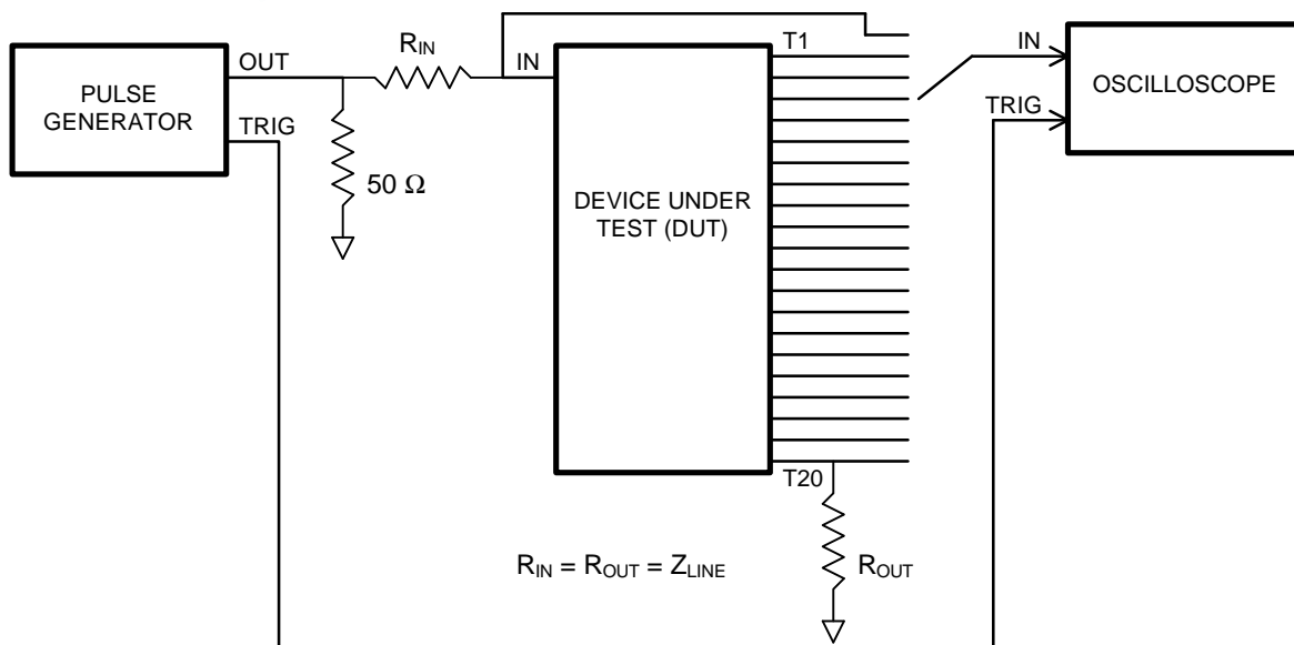
Test Setup
