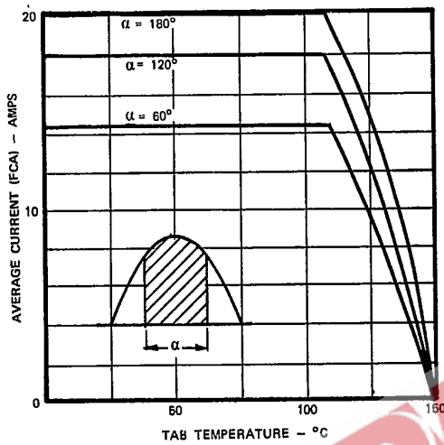
Fig. 1 - Forward Current Vs. Tab Temperature
