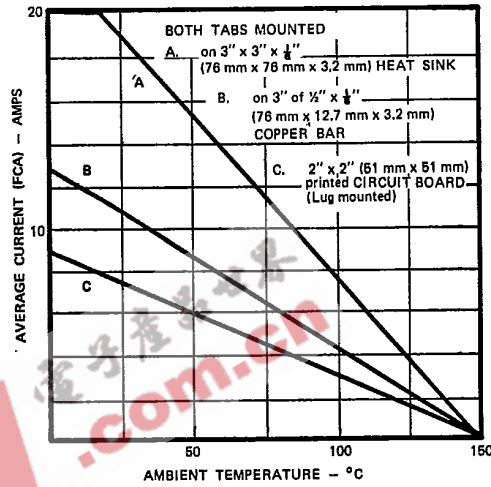
Fig. 2 - Forward Current Vs. Ambient Temperature
