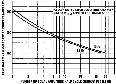
Fig. 9 - Maximum Non-Repetitive Surge Current Vs. Number of Current Pulses, 4AF Series
