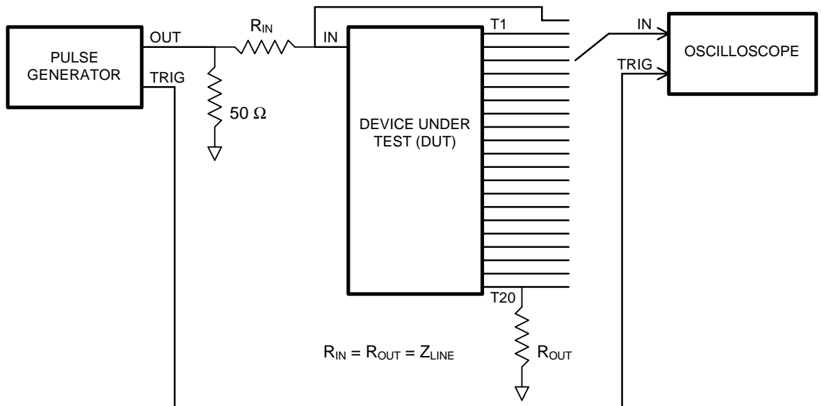
Test Setup
