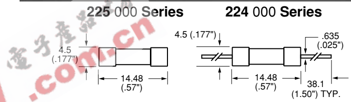
Axial Lead Material: Solder coated copper.
