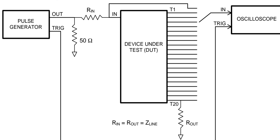
Test Setup
