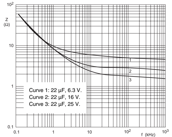
Fig.8 Typical impedance as a function of frequency at 20 ^{\circ}\text{C} .
