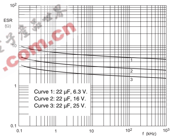
Fig.6 Typical ESR as a function of frequency at 20 ^{\circ}\text{C} .
