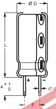
Fig.3 Form CB: Cut leads.
