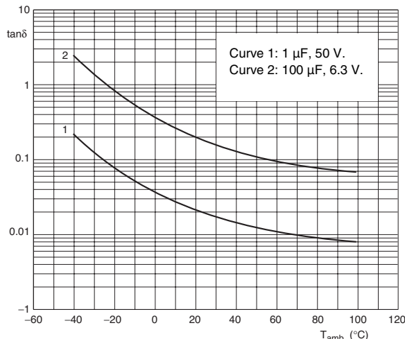
Fig.7 Typical dissipation factor (tan δ) at 100 or 120 Hz as a function of ambient temperature.
