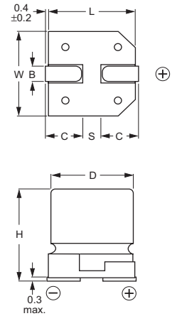
Fig.2 Dimensional outline.
