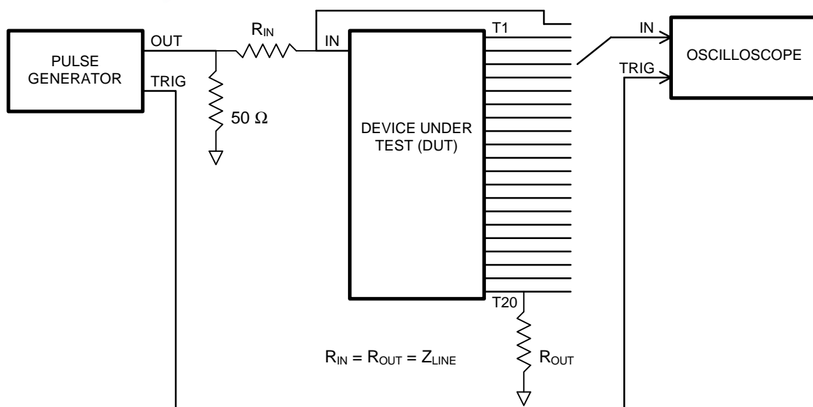
Test Setup
