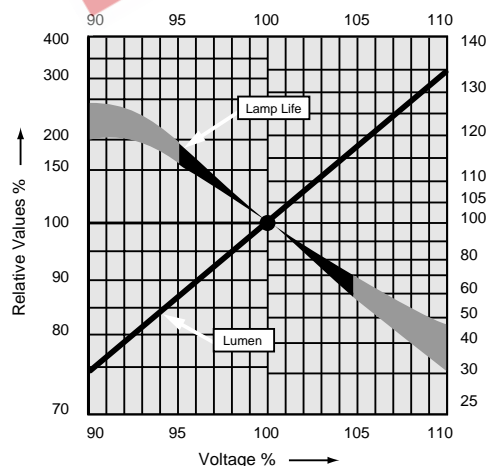
Life/Lumen-Volt Characteristic
