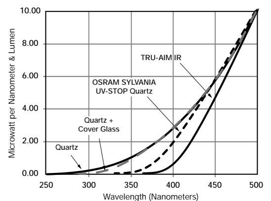
UV-Transmission Curves of Quartz Halogen Capsules
