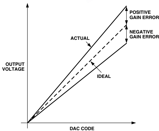
Figure 2. Gain Error
