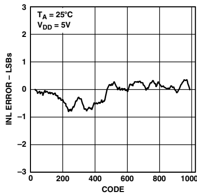
Figure 6. AD5333 Typical INL Plot
