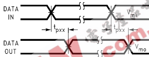
FIGURE 4. Waveform for Inverting and Non-Inverting Functions
