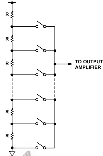
Figure 7. Resistor String
