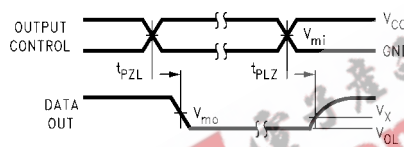
FIGURE 2. Waveform for Open Drain, Inverting and Non-inverting Functions
