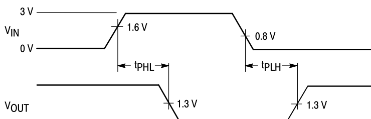
Figure 2. AC Waveforms
