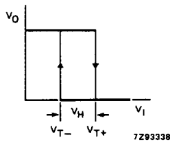
Fig.6 Transfer characteristic.
