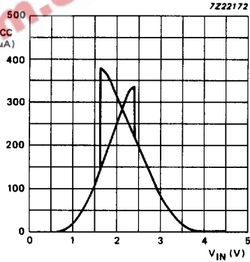
Fig.9 Typical HC transfer characteristics; V_{CC} = 4.5 \text{ V} .
