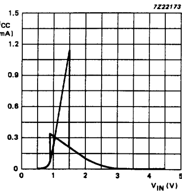
Fig.11 Typical HCT transfer characteristics; V_{CC} = 4.5 \text{ V} .
