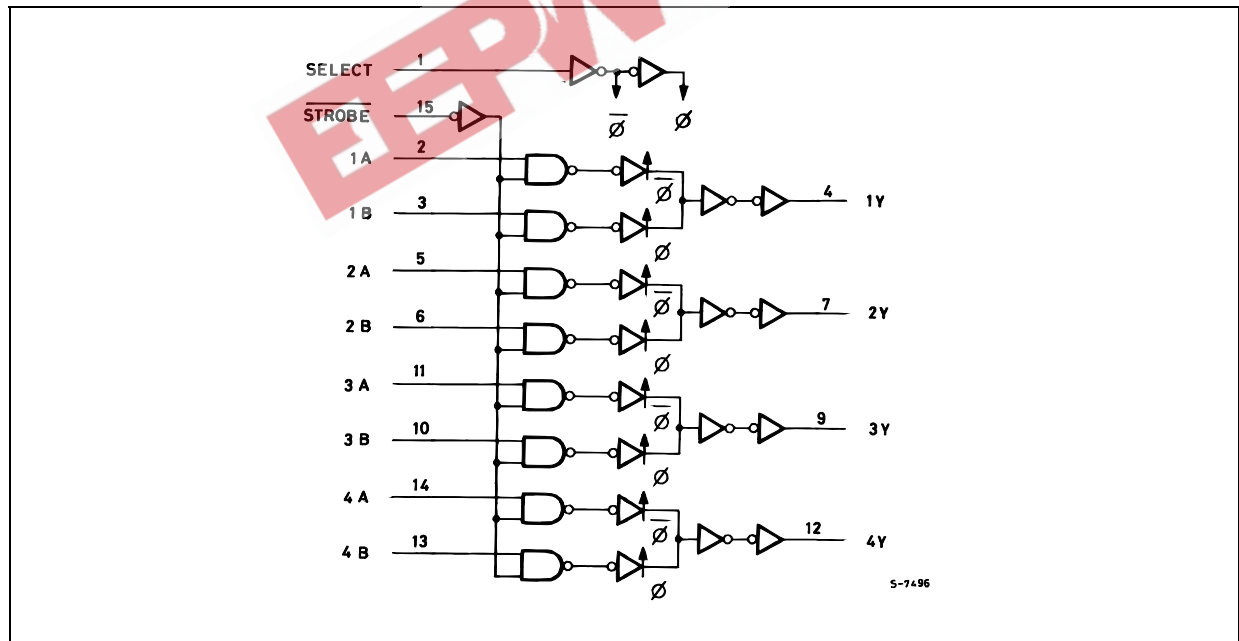
Figure 3: Logic Diagram
