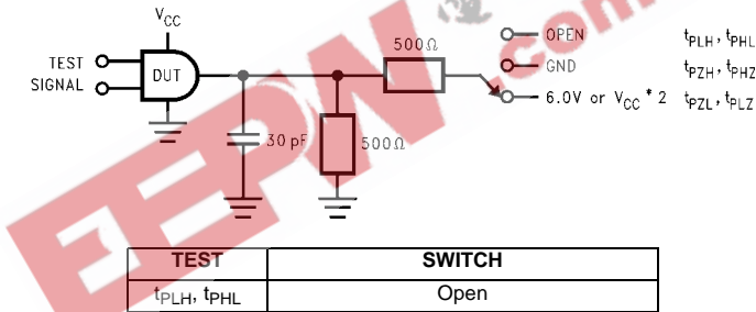
FIGURE 1. AC Test Circuit
