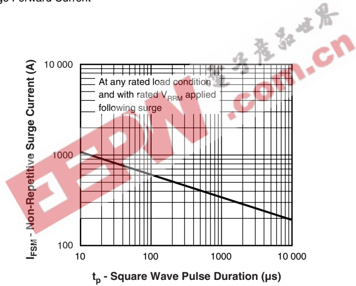
Fig. 7 - Maximum Non-Repetitive Surge Current (Per Leg)
