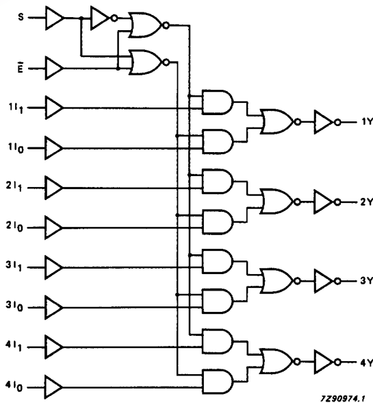
Fig.5 Logic diagram.
