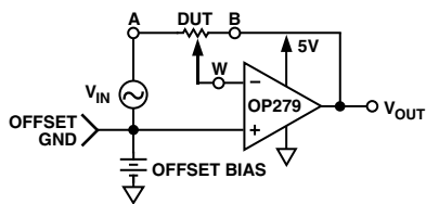
Figure 14. Inverting Gain Test Circuit
