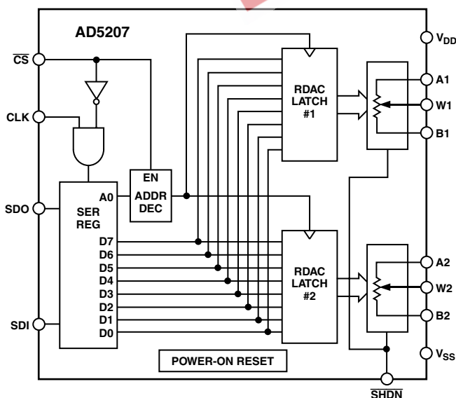
Figure 2. Block Diagram
