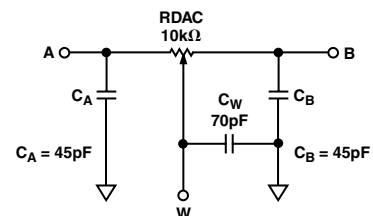
Figure 9. RDAC Circuit Simulation Model for RDAC = 10 kΩ
