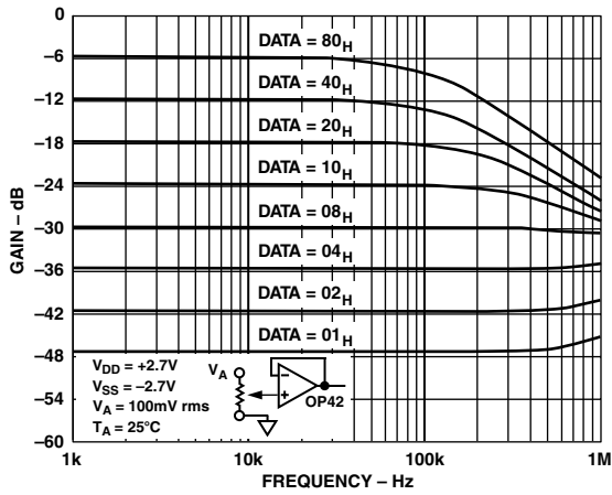
TPC 13. 50 kΩ Gain vs. Frequency vs. Code
