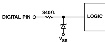
Figure 6. ESD Protection of Digital Pins
