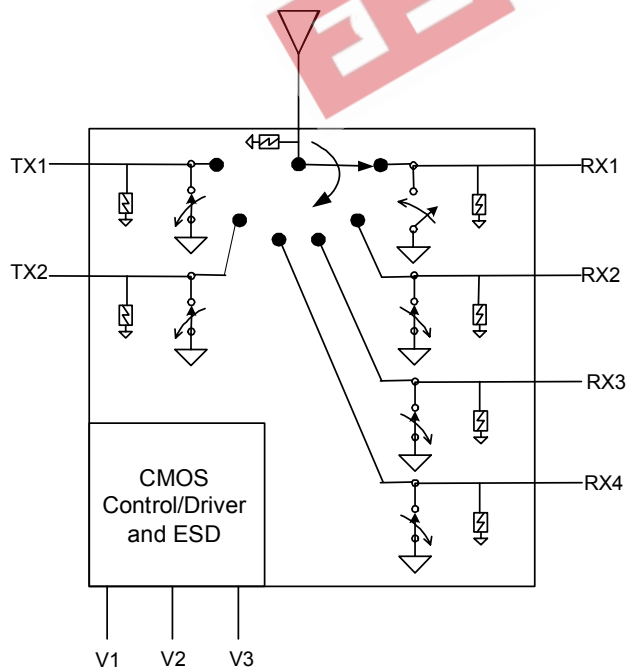
Figure 1. Functional Diagram
