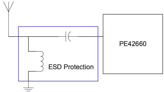
Figure 10. ESD Protection Circuit
