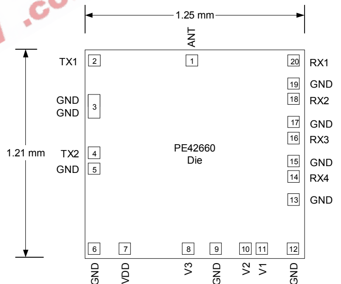
Figure 9. Pad Numbering
