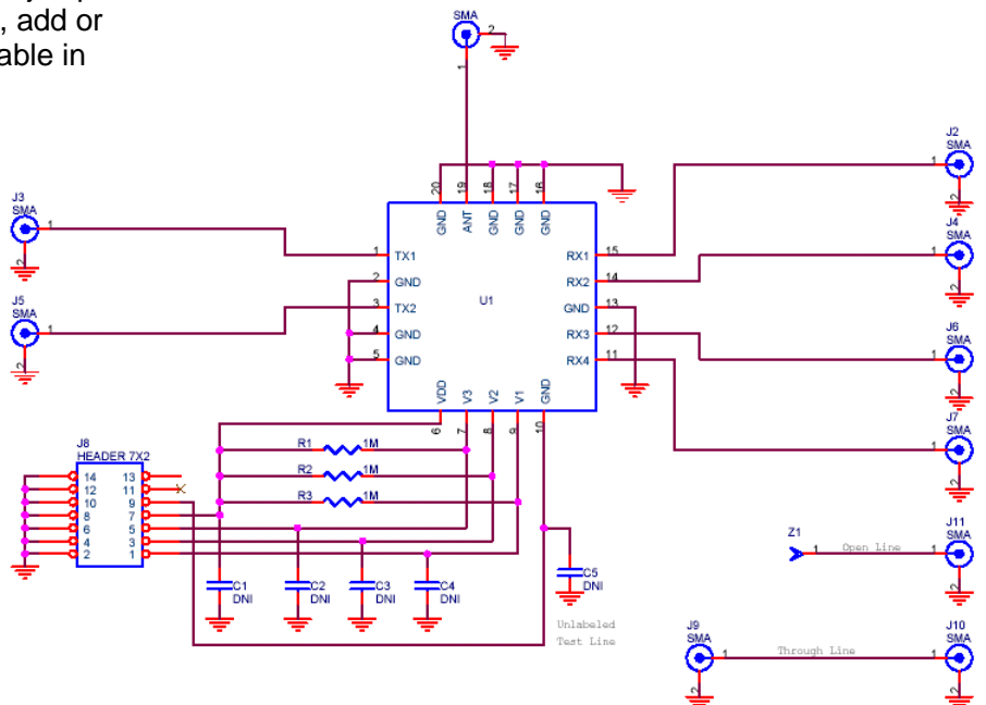
Figure 5. Evaluation Board Schematic Peregrine Specification 102/0267
