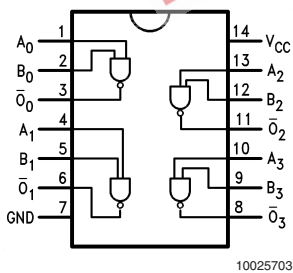
Pin Assignment for DIP and Flatpak
