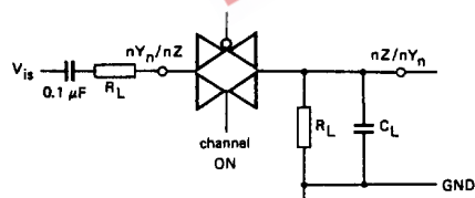
Fig.16 Test circuits for measuring crosstalk between any two switches/multiplexers.
