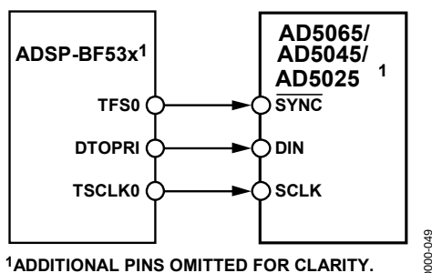
Figure 48. AD5025/45/65 to Blackfin ADSP-BF53X Interface
