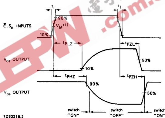
Fig.19 Waveforms showing the turn-ON and turn-OFF times.
