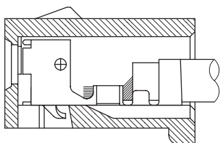
TERMINAL ASSEMBLY DRAWING
