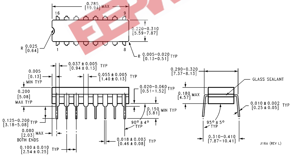
16-Lead Ceramic Dual-In-Line Package (J) Order Number 54LS155DMQB, 54LS156DMQB, DM54LS155J or DM54LS156J NS Package Number J16A
