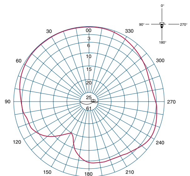
Vertical Directivity Pattern (90°)
