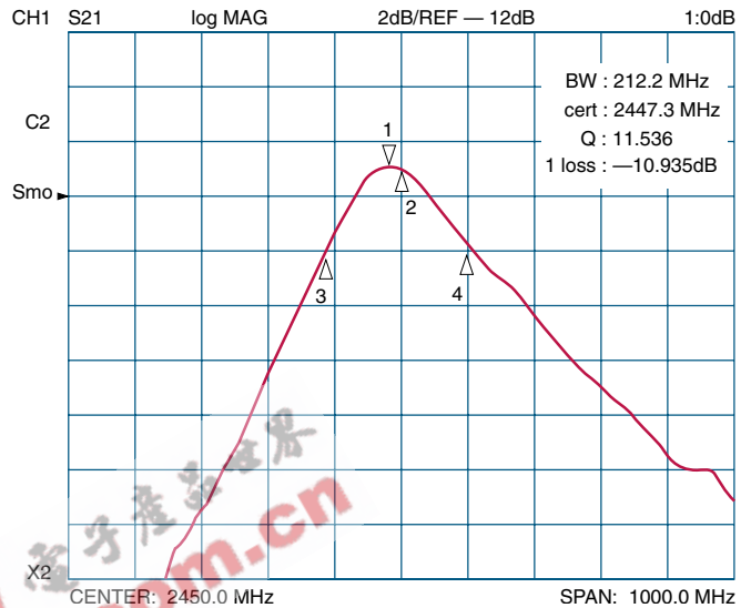
Receiving Signal Response Over Frequency
