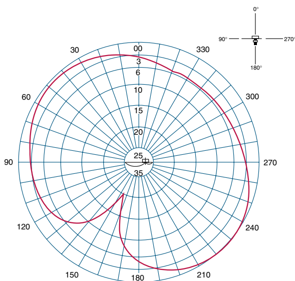
Vertical Directivity Pattern (0°)
