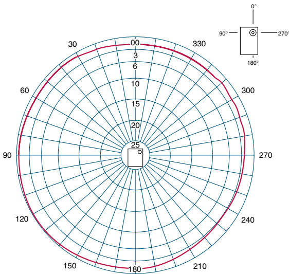
Horizontal Directivity Pattern
