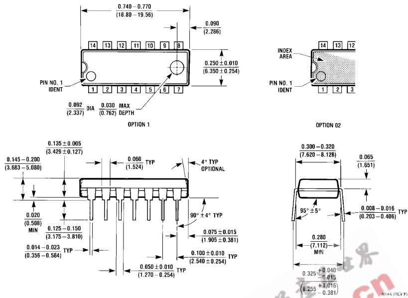
14-Lead Molded Dual-In-Line Package (N)
