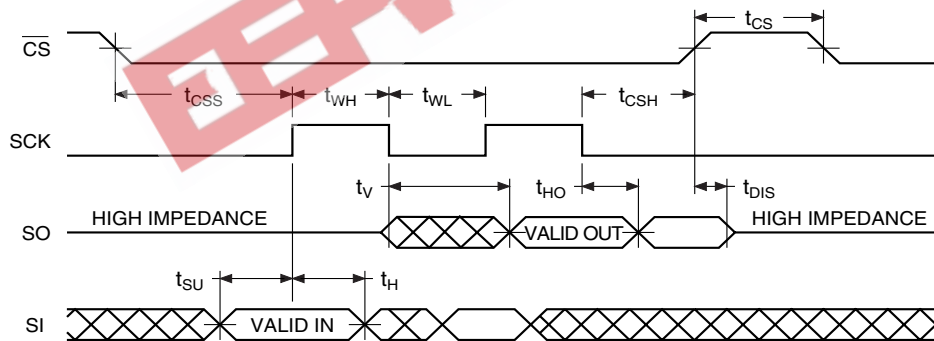
Waveform 3 – RapidS Mode 0 (for all Frequencies)
