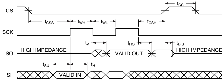
Waveform 1 – SPI Mode 0 Compatible (for Frequencies up to 33 MHz)
