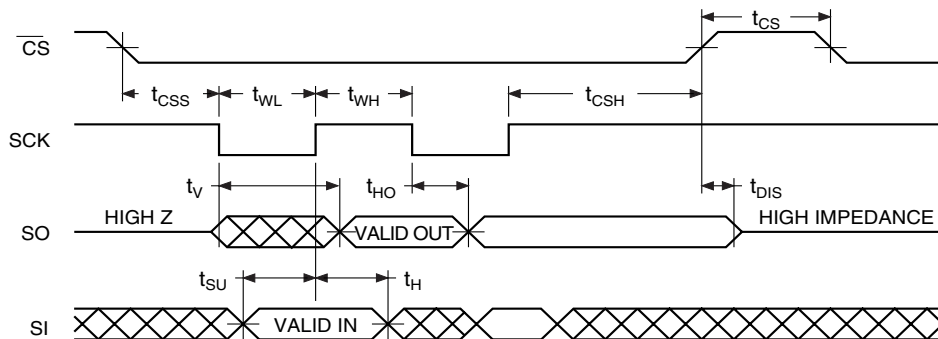
Waveform 4 – RapidS Mode 3 (for all Frequencies)
