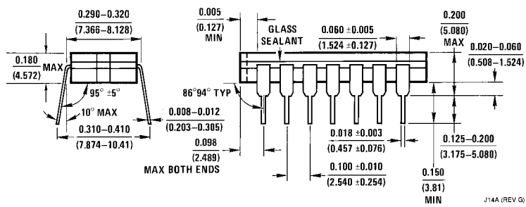
14-Lead Ceramic Dual-In-Line Package (J) Order Number 54LS32DMQB or DM54LS32J NS Package Number J14A
