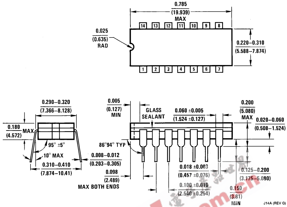
14-Lead Ceramic Dual-In-Line Package (J) Order Number DM54LS55J NS Package Number J14A
