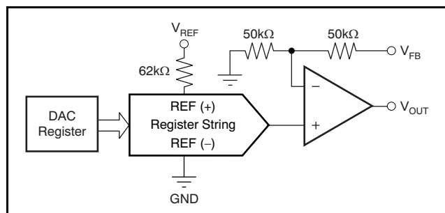
Figure 62. DAC8560 Architecture
