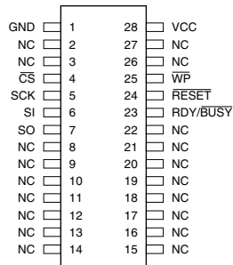
Figure 2-4. 28-SOIC (1)
