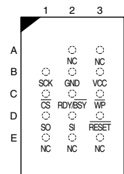
Figure 2-5. CBGA Top View through Package
