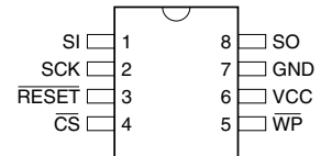
Figure 2-2. 8-SOIC
