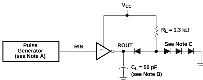
TEST CIRCUIT
