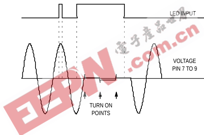
Figure 11. Operating Waveforms
