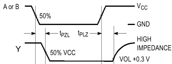
Figure 4. Switching Waveforms
